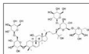
Mogroside V
