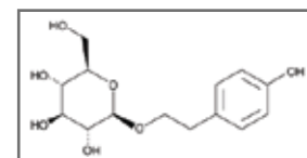
Salidroside CAS #: 10338-51-9
