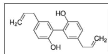
Magnolol CAS #: 528-43-8
