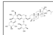
Jujuboside B CAS #: 55466-05-2
