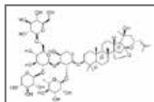
Jujuboside A CAS #: 55466-04-1
